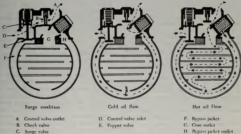
FIGURE 6-6. Control valve with surge protection.
